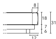
Ecoveneer plinth with additional feet
