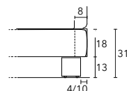
Plinth with feet 13 cm H
