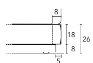
Ecoveneer plinth with concealed adjustable feet
