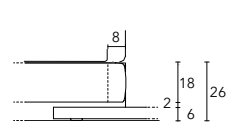
Plinth sitting on platform
