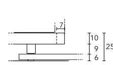
Plinth with feet sitting on platform
